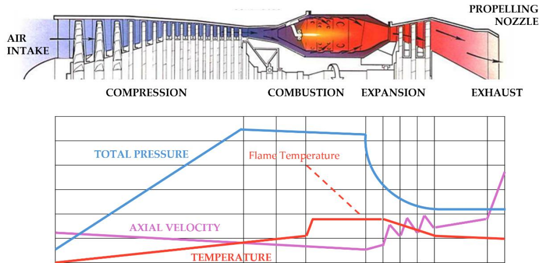
Figure 8: Pressure, velocity, and temperature profile across jet engines (Adapted by author from Rolls-Royce plc 1996). 24
