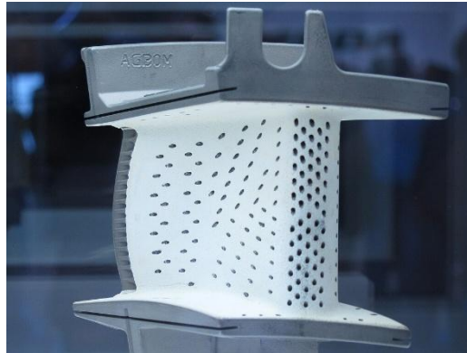
Figure 16: Laser-drilled holes permit film cooling. 25
