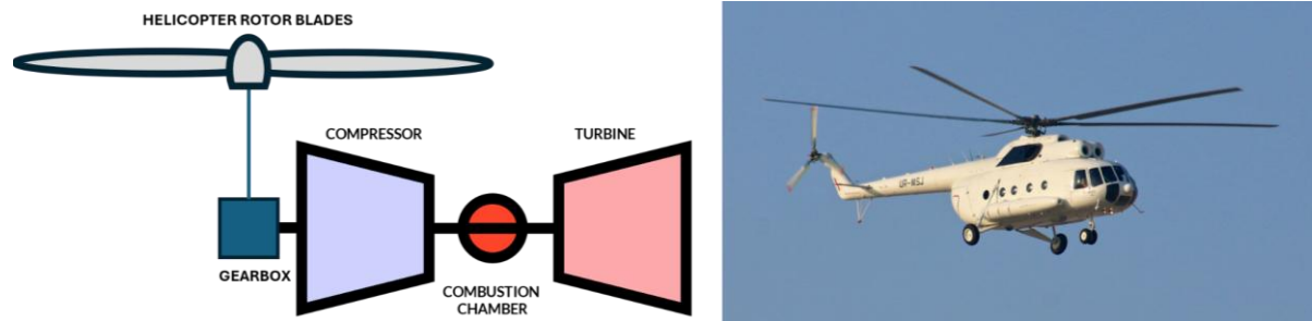
Figure 11: Block diagram and application of turboshaft (Unsplash n.d.). 7
