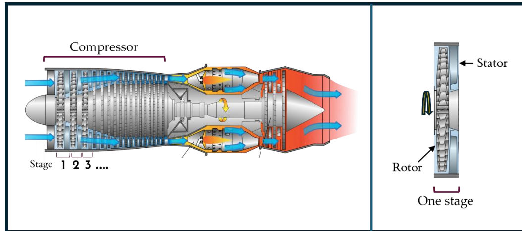
Figure 6: Stages in an axial compressor. 24
