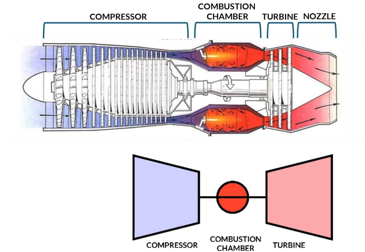
Figure 4: Block diagram of three main components of a jet engine. 24
