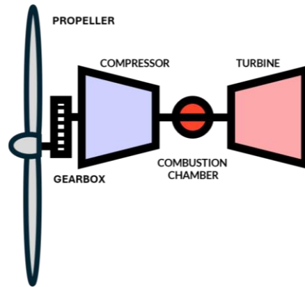
Figure 9: Block diagram and application of turboprop (Unsplash n.d.). 7
