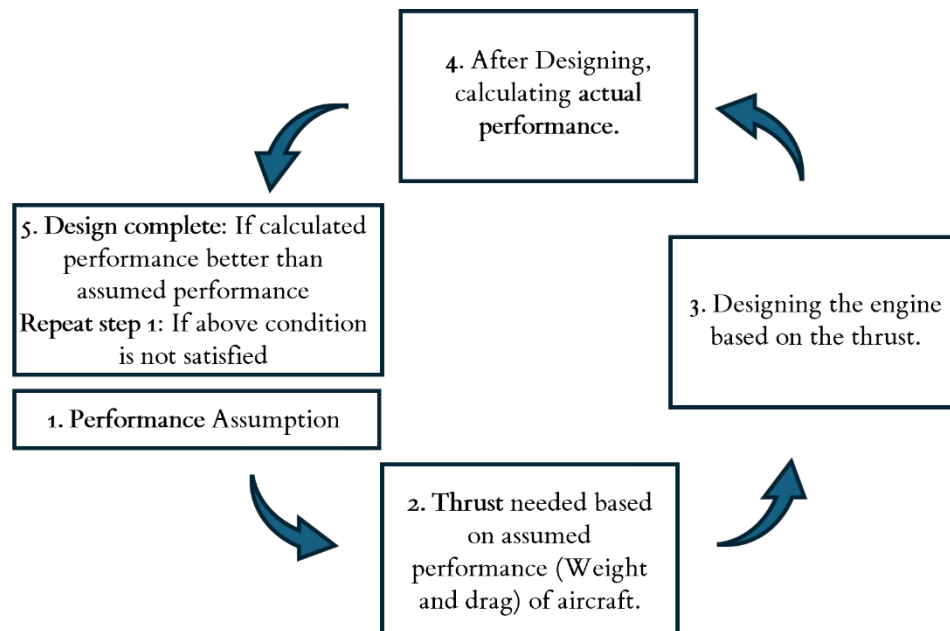
Figure 13: A representation of the iterative engine design process. (Collated/ Created by Author)
